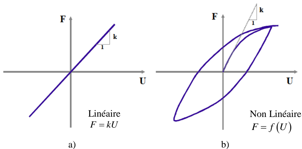
Figure 1.2 : Relation force-déplacement [1]
