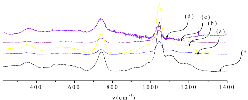
Figure III-5 : Spectres de Raman de verres
